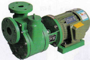
FP系列耐腐蚀自吸泵(直接式) Plastics centrifgal plastics pump(direct-like)
