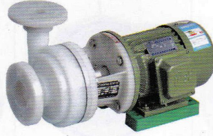
FV系列耐腐蚀离心泵(直接式) Corrosion resisting plastics centrifgal pump (direct-like)
