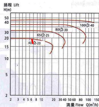
FZ系列耐腐蚀自吸泵谱图 FZ self-suction pump flow graph:
