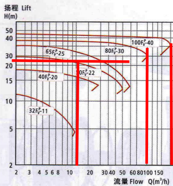
F系列耐腐蚀离心泵 F Centrifugal pump flow graph:
